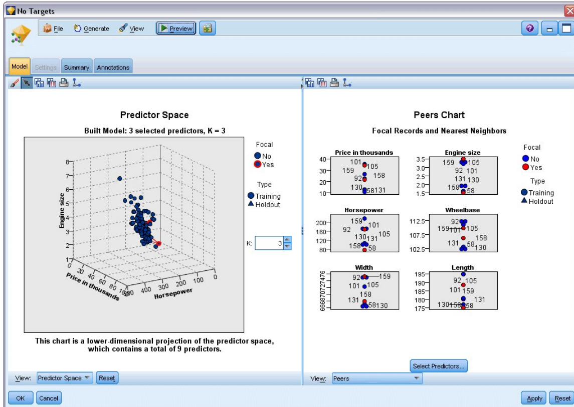
Figura 391. La ventana Model Viewer
